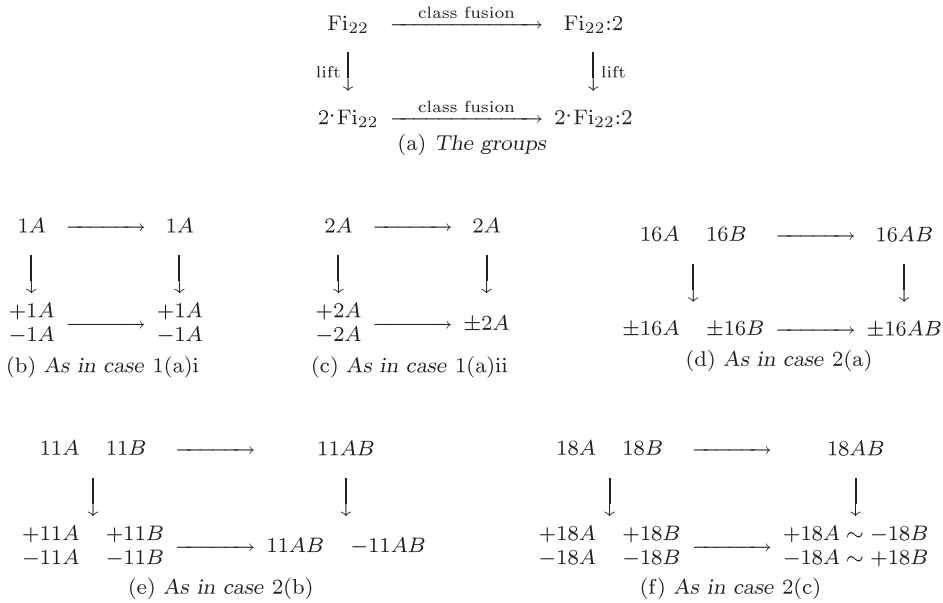
FIGURE 1. The relationship between conjugacy classes of \text{Fi}_{22} and 2 \cdot \text{Fi}_{22}:2 . Horizontal arrows are for class fusion under the automorphism, and vertical arrows show lifting to the double cover. Diagram (a) shows the groups involved. The other diagrams give examples of some of the possibilities. Class names are for \text{Fi}_{22} .
