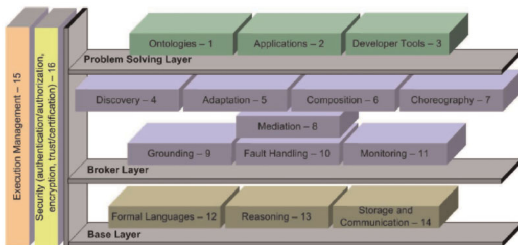
Fig. 7. The internal architecture of a semantic execution environment. [A color version of this figure can be viewed online at journals.cambridge.org/aie]
