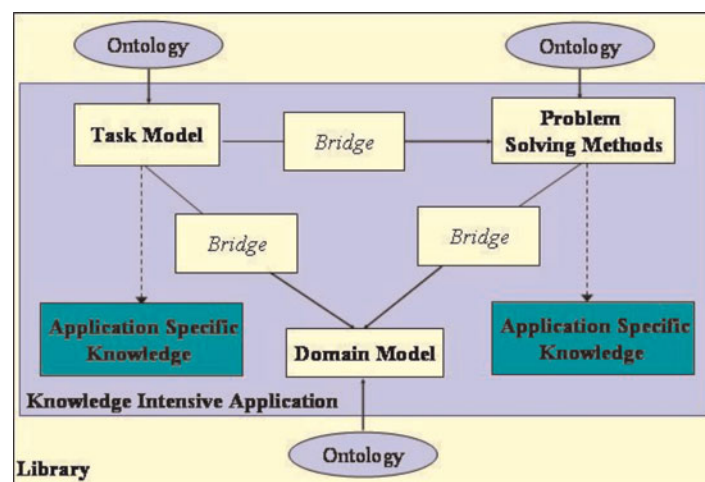
Fig. 2. The UPML framework. [A color version of this figure can be viewed online at journals.cambridge.org/aie ]
