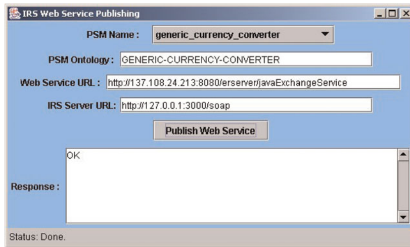
Fig. 5. The interface for the IRS-II Web service publisher. [A color version of this figure can be viewed online at journals.cambridge.org/aie ]
