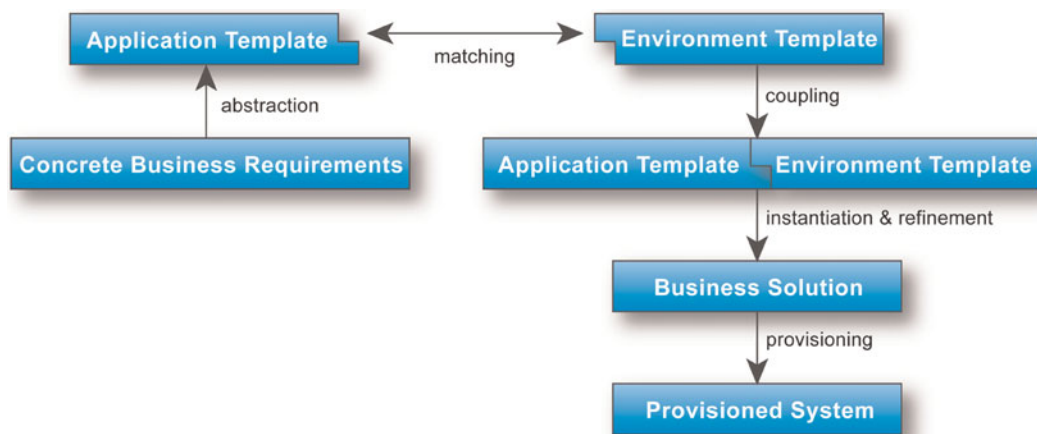
Fig. 8. A heuristic classification based life cycle for transforming business applications into utilities. [A color version of this figure can be viewed online at journals.cambridge.org/aie ]
