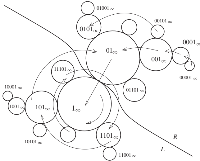
FIGURE 2. Example of itineraries of \Delta and of pullbacks of \Delta' and of their dynamics for the golden mean basic Siegel Julia set. Some of the missing arrows can be determined by using the central symmetry: two symmetric components are mapped to the same component.
